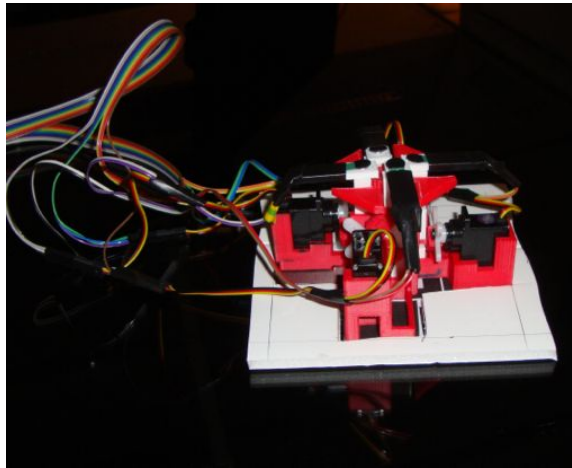
Figure 7.2: HaptiQ with extended white board base
