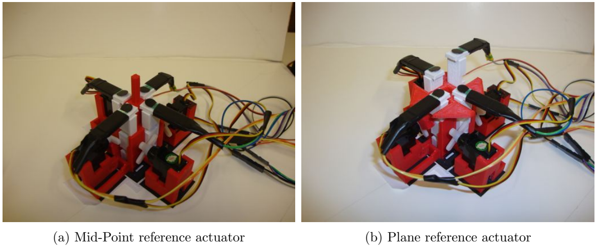
Figure 6.3: HaptiQ reference static actuators
