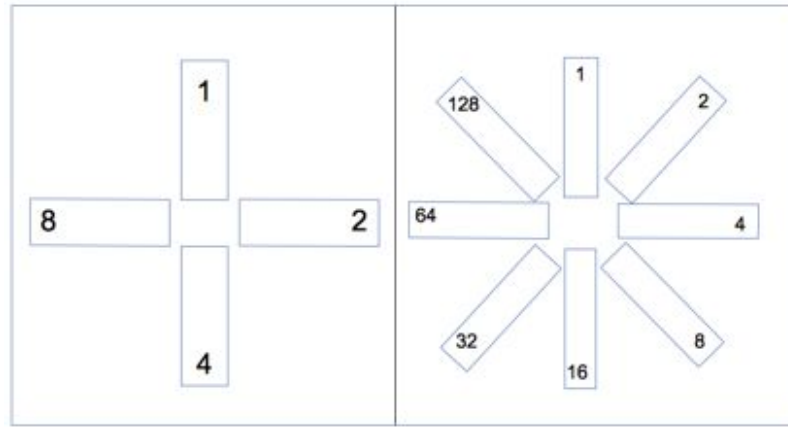
Figure 7.5: Actuators bits representation
