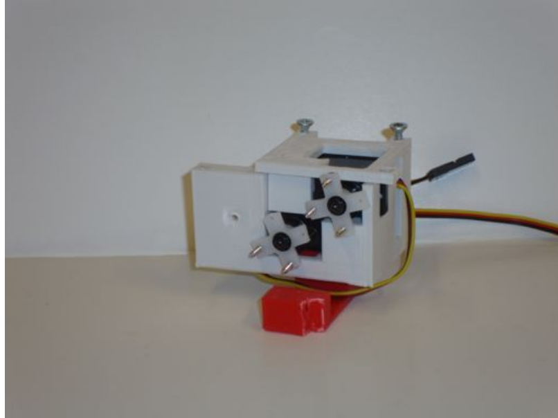
Figure 6.5: 8-HaptiQ servos couple
