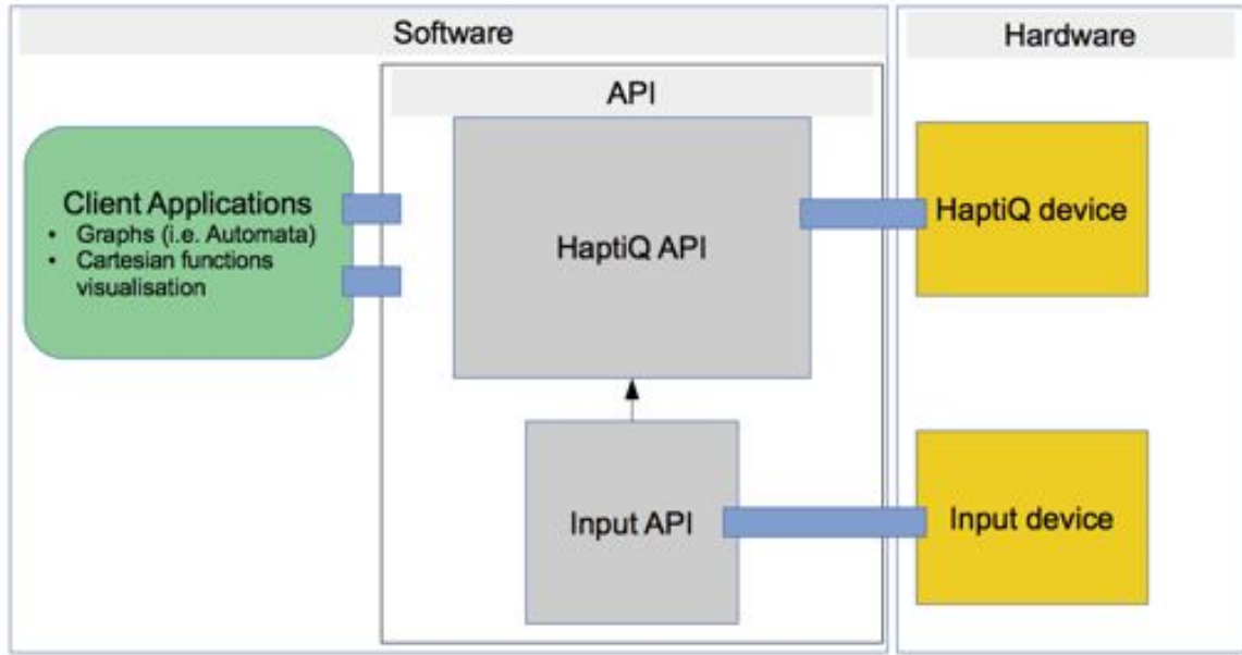
Figure 6.8: API General Overview
