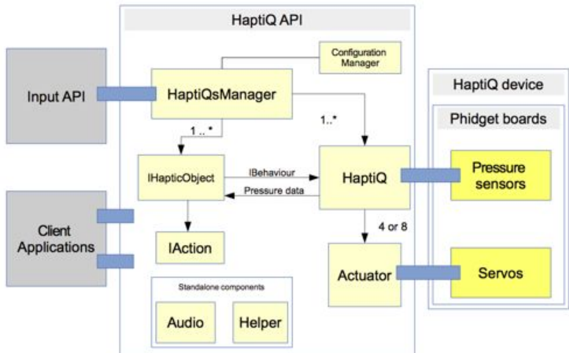
Figure 6.10: HaptiQ API
