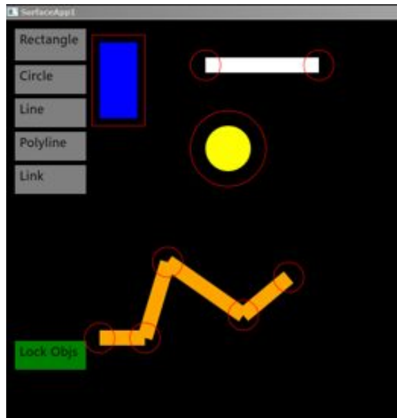
Figure 6.18: Graph Visualiser
