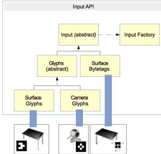
Figure 6.9: Input API
