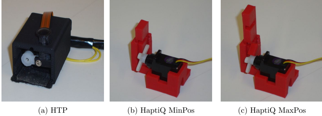
Figure 6.2: HTP and HaptiQ actuator mechanics
