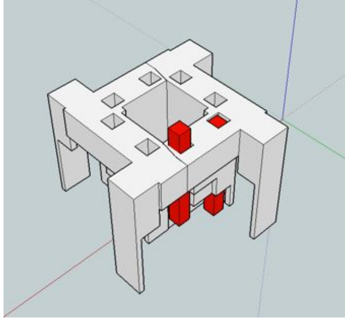
Figure 6.6: 8-HaptiQ reference plane and actuators slots
